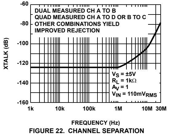
FIGURE 22. CHANNEL SEPARATION
