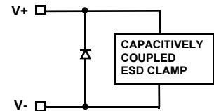
CIRCUIT 3
