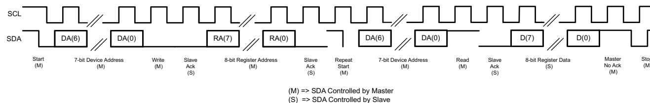
Figure 5-53. I²C Read
