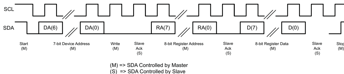
Figure 5-52. I²C Write
