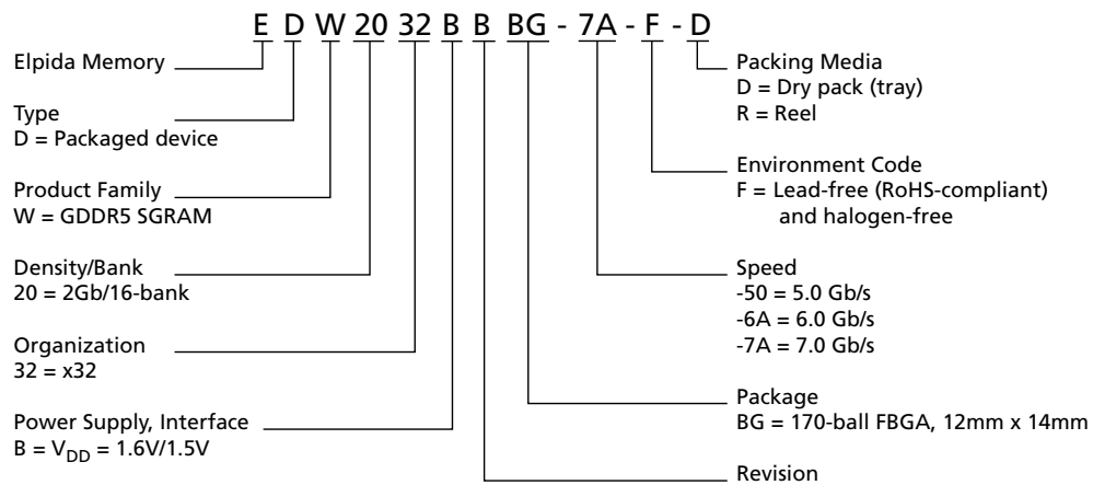
Figure 1: Part Numbering
