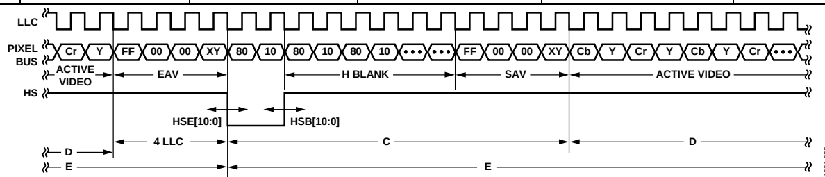
Figure 31. HSYNC Timing Rev. C | Page 42 of 96
