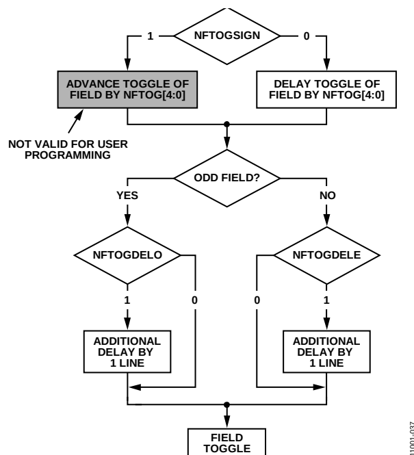
Figure 36. NTSC FIELD Toggle
