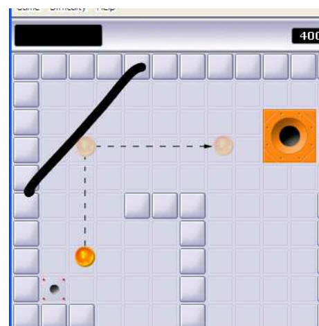
Figure 38. Game
