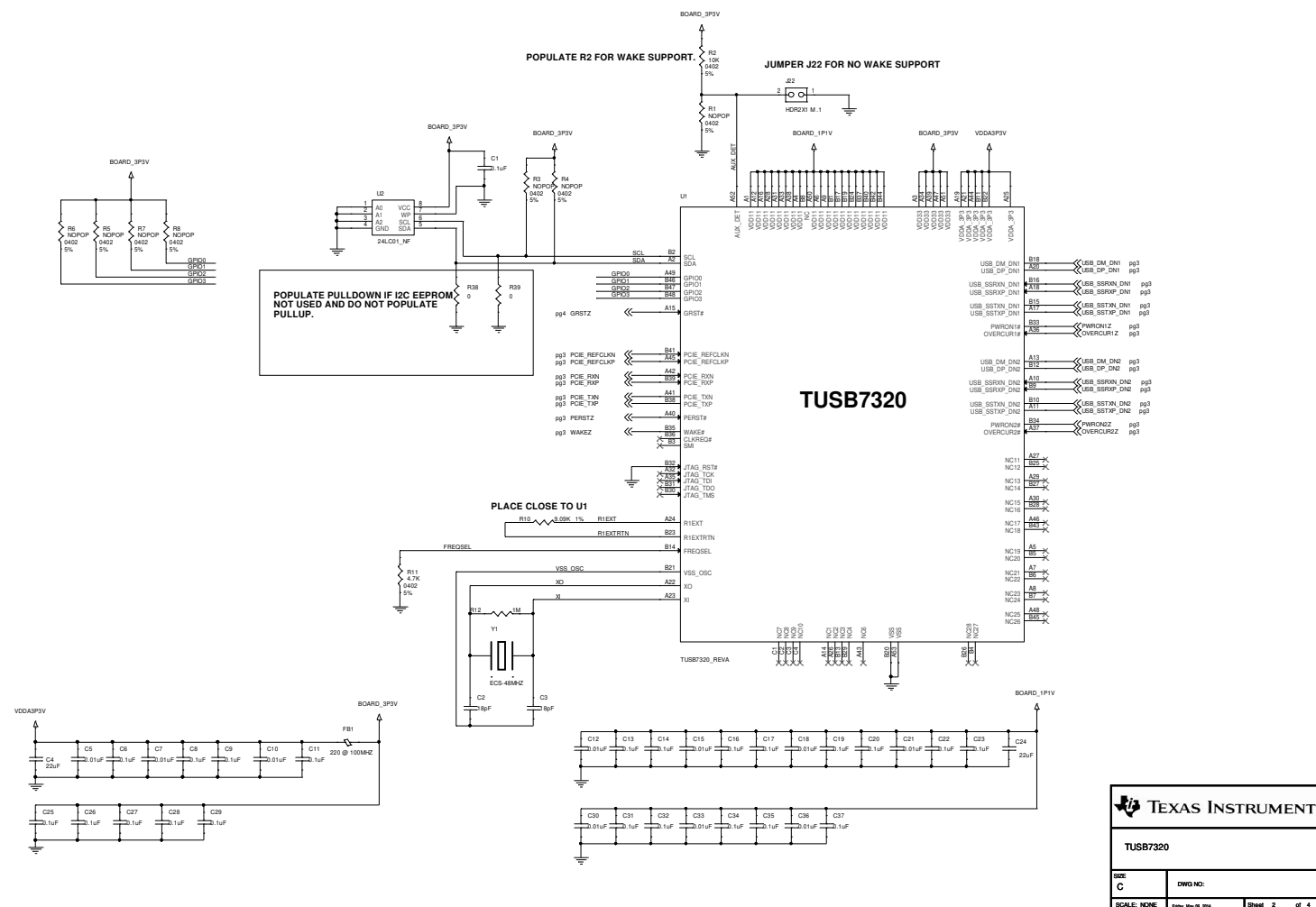
Figure 7-3. Reference Design 1
