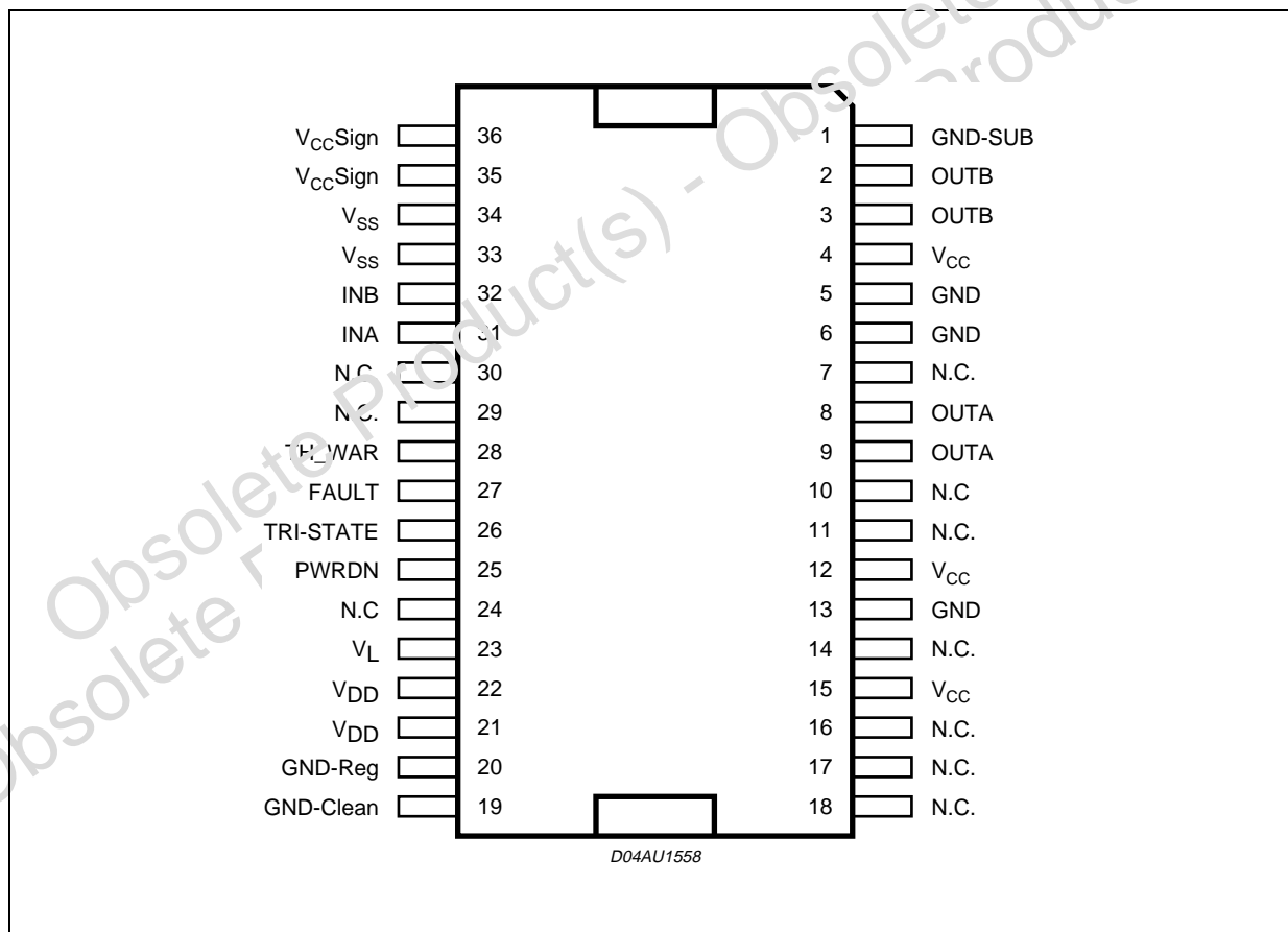
Figure 4. PIN CONNECTION
