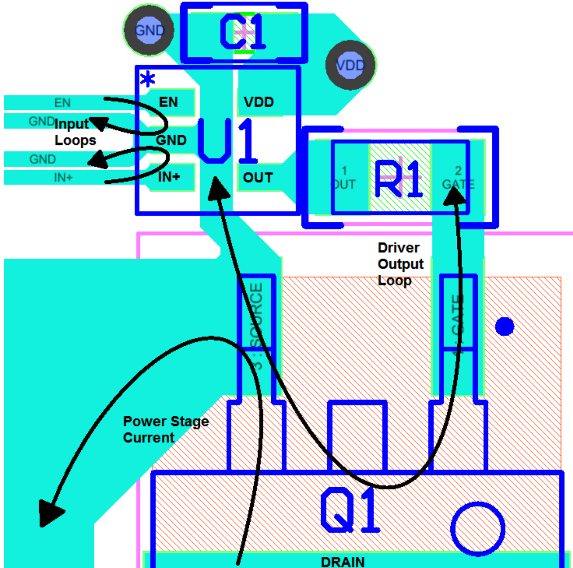
Figure 26. Layout Example
