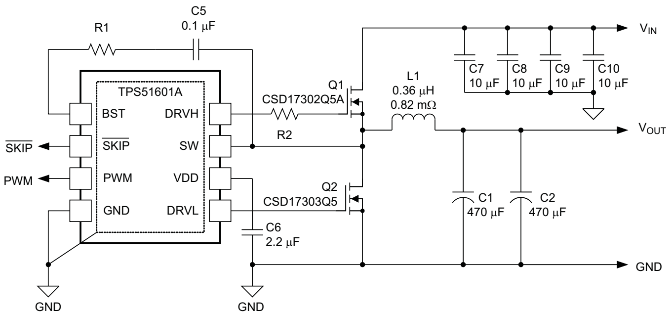
Figure 19. Typical Application
