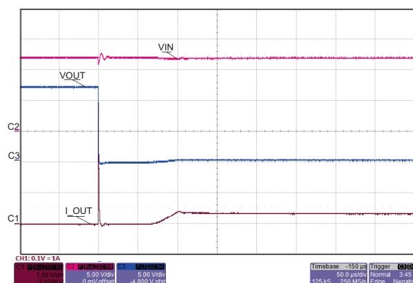
Transient: Output Short Circuit
