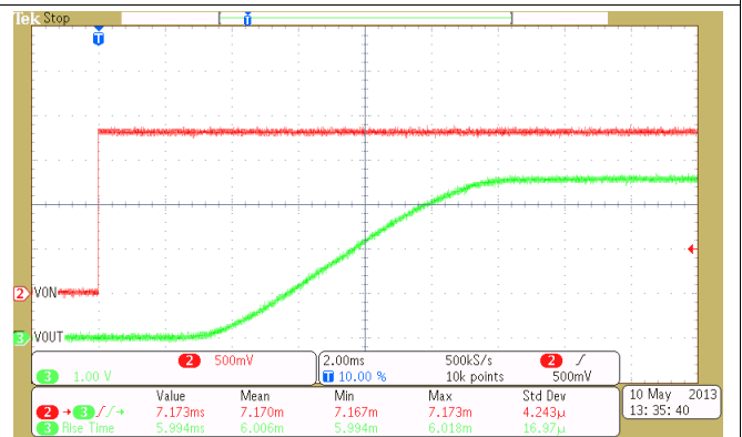
Figure 24. Turnon Response ( C_{IN} = 10 \mu F, C_L = 1 \mu F, R_L = 10 \Omega, V_{IN} = 3.6 V, T_A = 25^\circ C )
