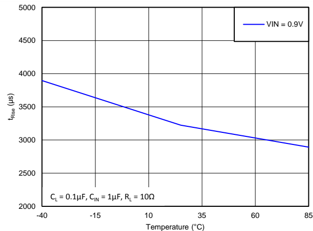
Figure 12. Rise Time vs Temperature (V IN = 0.9 V, C L = 0.1 μF, R L = 10 Ω)
