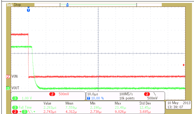
Figure 23. Turnoff Response ( C_{IN} = 1 \mu F, C_L = 0.1 \mu F, R_L = 10 \Omega, V_{IN} = 3.6 V, T_A = 25^\circ C )
