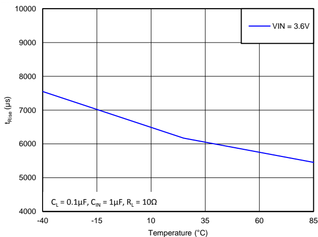
Figure 8. Rise Time vs Temperature (V IN = 3.6 V, C L = 0.1 μF, R L = 10 Ω)
