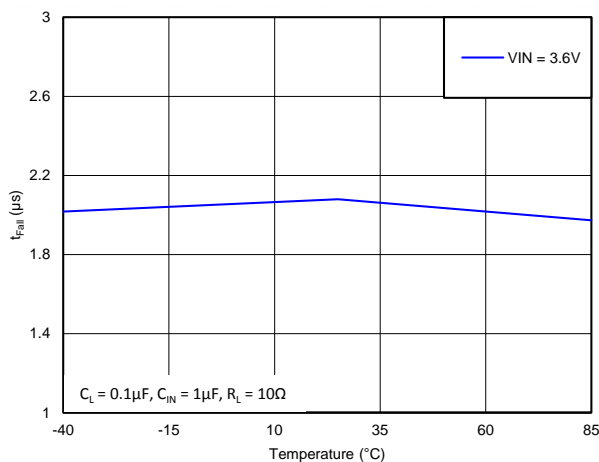
Figure 9. Fall Time vs Temperature (V IN = 3.6 V, C L = 0.1 μF, R L = 10 Ω)
