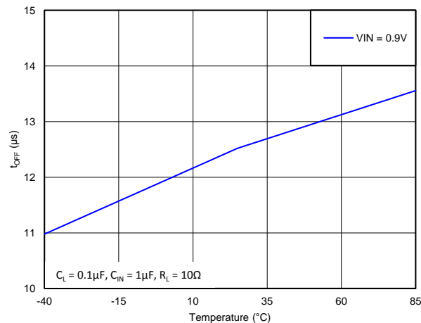
Figure 11. Turnoff Time vs Temperature (V IN = 0.9 V, C L = 0.1 μF, R L = 10 Ω)
