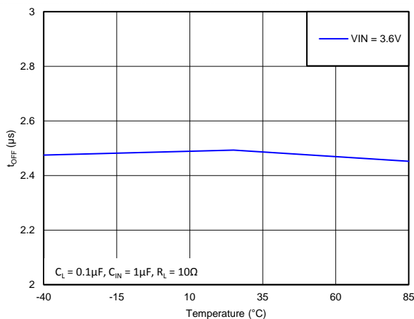
Figure 7. Turnoff Time vs Temperature (V IN = 3.6 V, C L = 0.1 μF, R L = 10 Ω)
