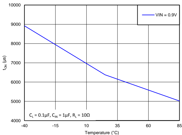
Figure 10. Turnon Time vs Temperature (V IN = 0.9 V, C L = 0.1 μF, R L = 10 Ω)
