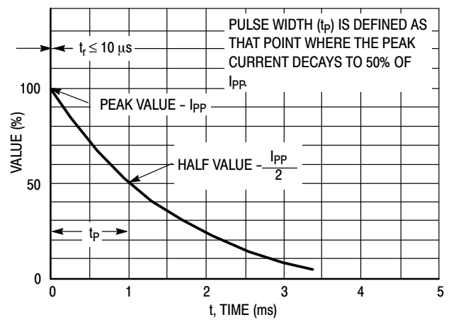
Figure 2. Pulse Waveform
