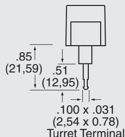
2 – Turret Type Solder Terminal
