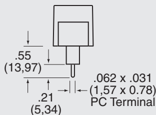
1 – Printed Circuit Pin
