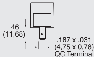
4 – Quick Connect .187"
