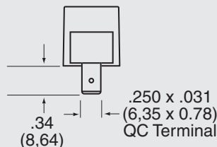
5 – Quick Connect .250"
