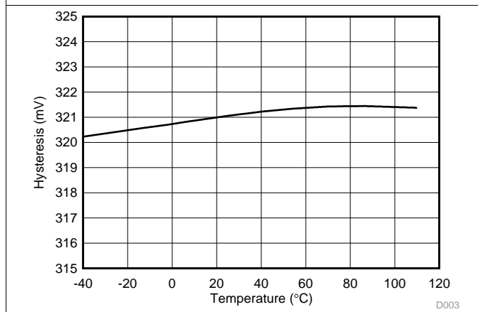
Figure 3. Hysteresis V HYS vs Temperature
