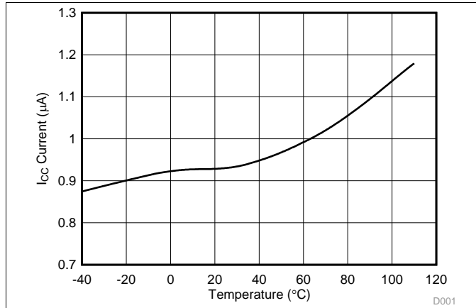
Figure 1. I CC Current Consumption vs Temperature
