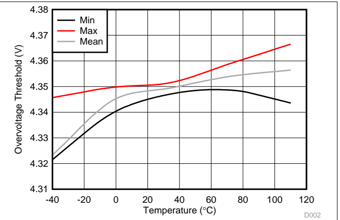
Figure 2. bq294602 Overvoltage Threshold (OVT) vs Temperature
