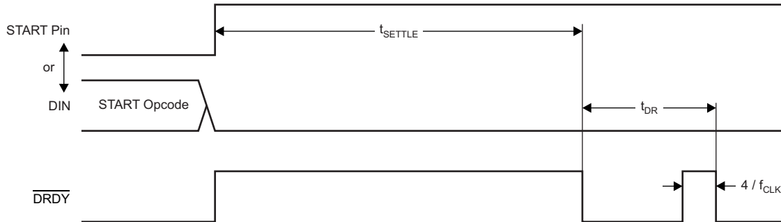
Figure 37. Settling Time
