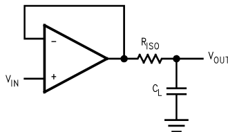
Figure 45. Isolating Capacitive Load
