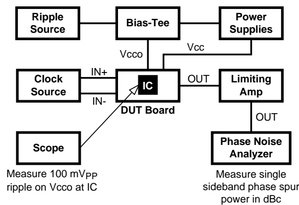
Figure 22. PSRR Test Setup
