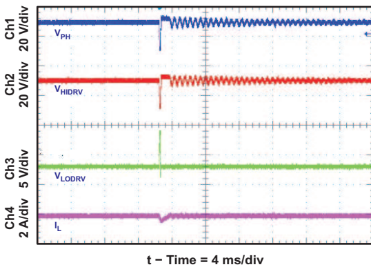
Figure 27. Nonsynchronous to Synchronous Transition
