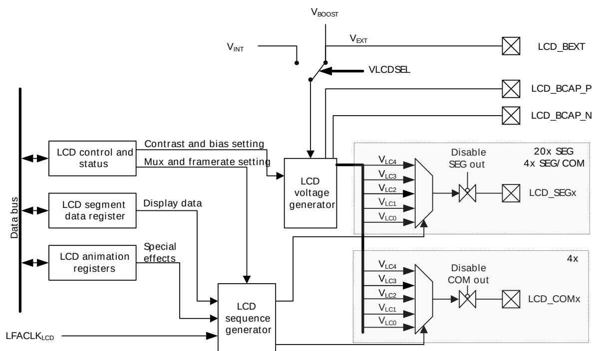
Figure 29.1. LCD Block Diagram
