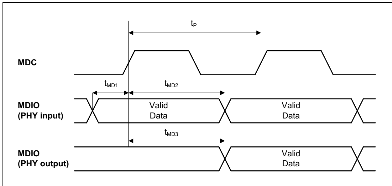
FIGURE 7-11: MDC/MDIO TIMING
