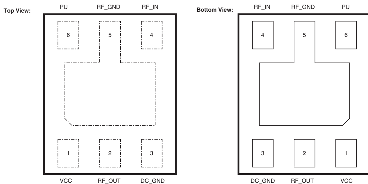
Figure 2-1. Pinning PLLP6 (Not Scaled)
