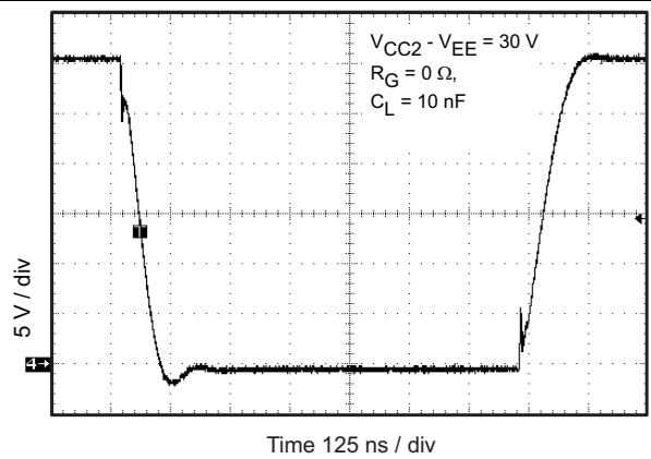
Figure 26. Output Waveform
