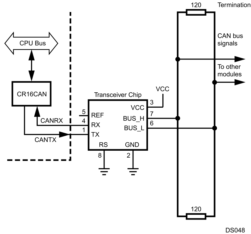
Figure 19-31. External Transceiver
