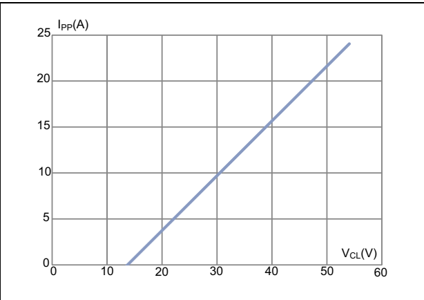
Figure 6. TLP measurements
