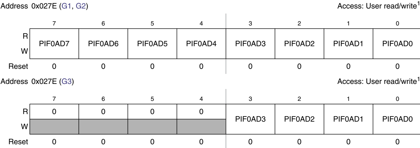
Figure 2-62. Port AD Interrupt Flag Register (PIF0AD)
