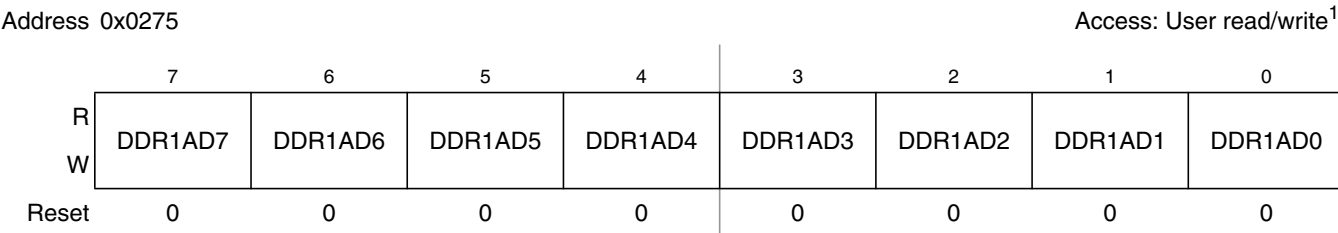
Figure 2-54. Port AD Data Direction Register (DDR1AD)
