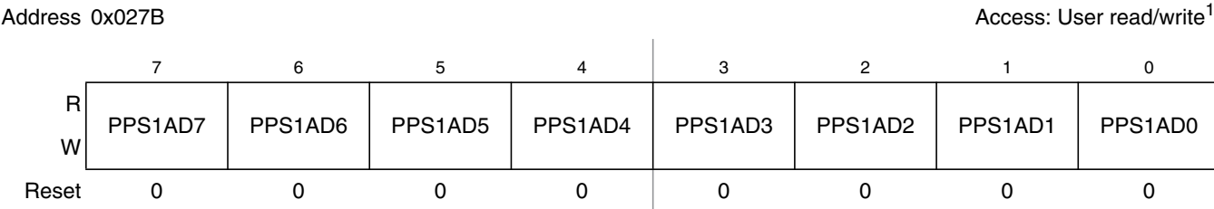
Figure 2-59. Port AD Polarity Select Register (PPS1AD)
