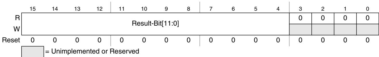
Figure 16-14. Left justified ATD conversion result register (ATDDRn)
