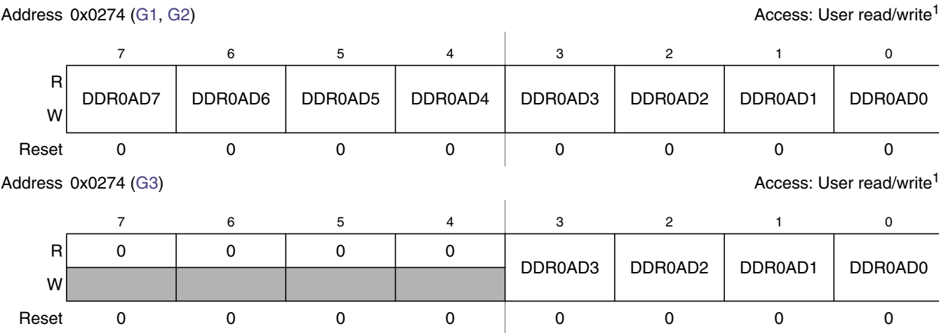
Figure 2-53. Port AD Data Direction Register (DDR0AD)
