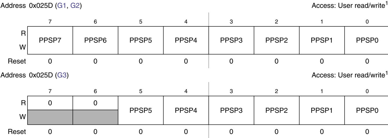
Figure 2-39. Port P Polarity Select Register (PPSP)
