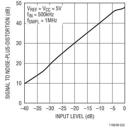
S/(N + D) vs Input Level
