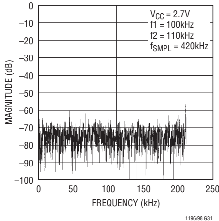
Intermodulation Distortion at 2.7V
