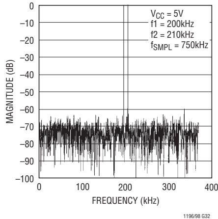
Intermodulation Distortion at 5V
