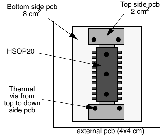
Figure 3. .Printed Board Layout Example (not to scale)
