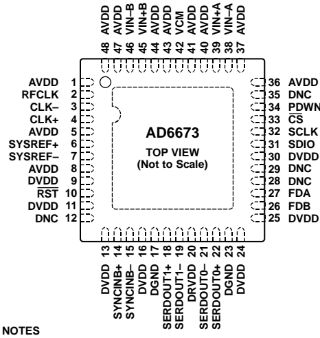
Figure 4. Pin Configuration (Top View)
