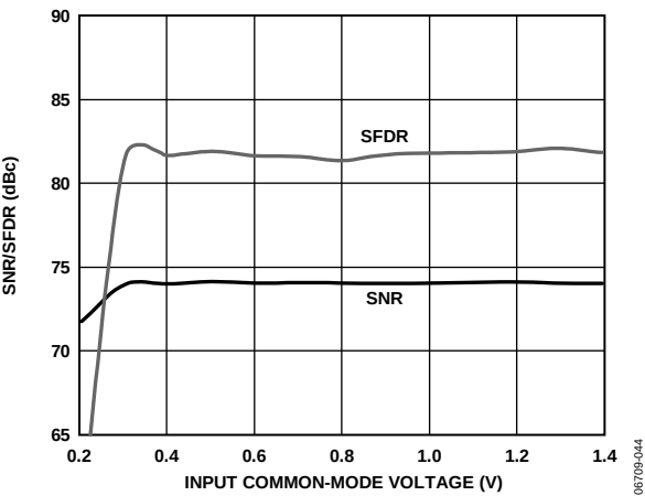
Figure 45. AD6655-150 SNR/SFDR vs. Input Common Mode ( V_{CM} ) with f_{IN} = 30.3\text{ MHz} , f_{NCO} = 45\text{ MHz}
