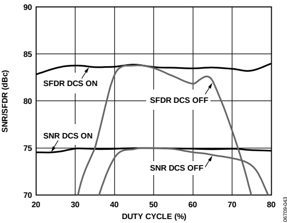
Figure 44. AD6655-150 SNR/SFDR vs. Duty Cycle with f_{IN} = 30.3\text{ MHz} , f_{NCO} = 45\text{ MHz}
