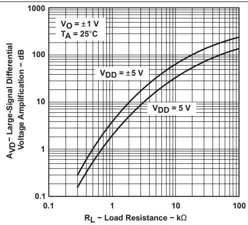
Figure 24. Large-Signal Differential Voltage Amplification vs Load Resistance
