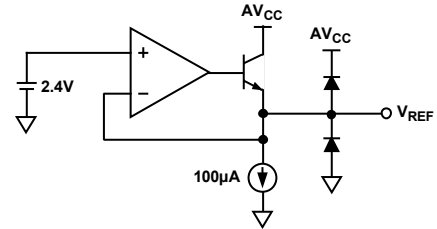
Figure 24. 2.4 V Reference
