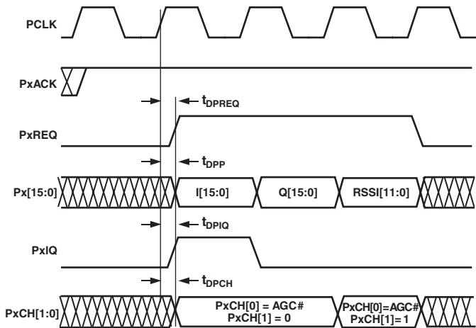
Figure 39. AGC Output with RSSI Word
