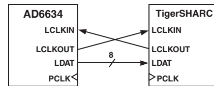
Figure 40. Link Port Connection between AD6634 and TigerSHARC
