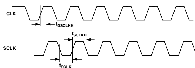
Figure 5. SCLK Switching Characteristics (Divide by 1)
