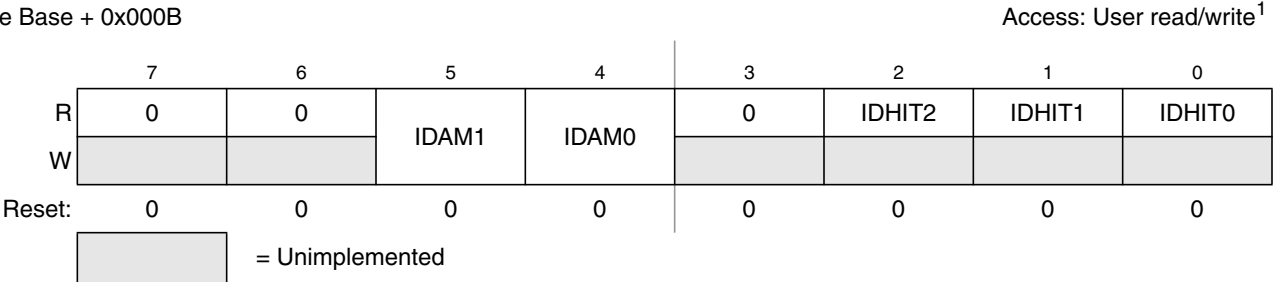
Figure 18-15. MSCAN Identifier Acceptance Control Register (CANIDAC)
