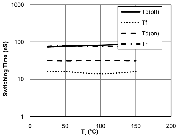
Figure 14: Switching Time vs. T_J ( V_{GE}=15\text{V}, V_{CE}=400\text{V}, I_C=60\text{A}, R_g=5\Omega )
