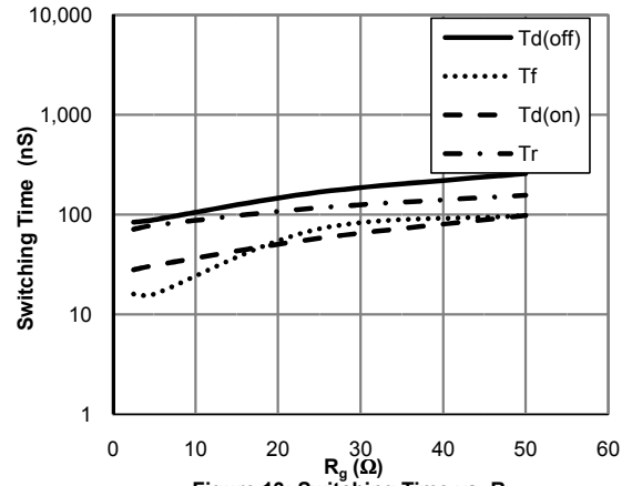
Figure 13: Switching Time vs. R_g ( T_J=150^{\circ}\text{C}, V_{GE}=15\text{V}, V_{CE}=400\text{V}, I_C=60\text{A} )
