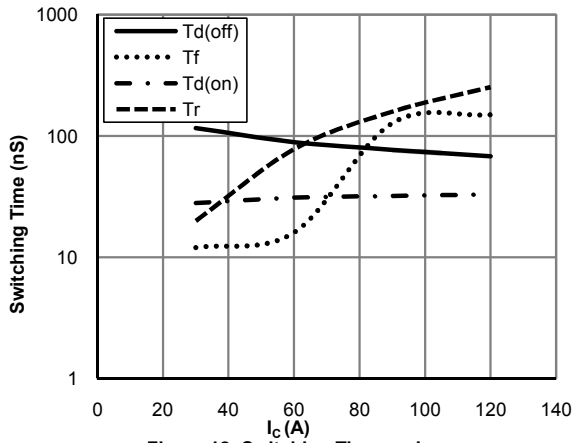
Figure 12: Switching Time vs. I_C ( T_J=150^{\circ}\text{C}, V_{GE}=15\text{V}, V_{CE}=400\text{V}, R_g=5\Omega )
