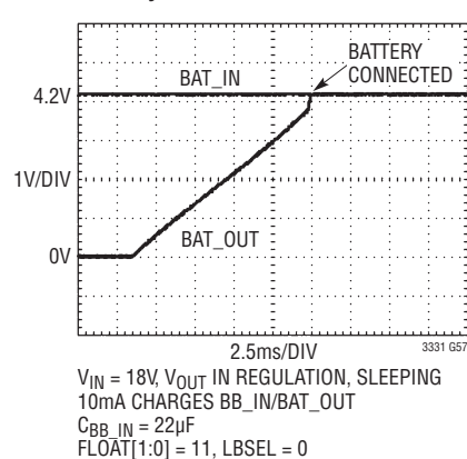
Battery Connect Transient
