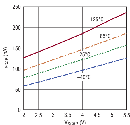
Supercapacitor Balancer Quiescent Current vs V_{\text{SCAP}}
