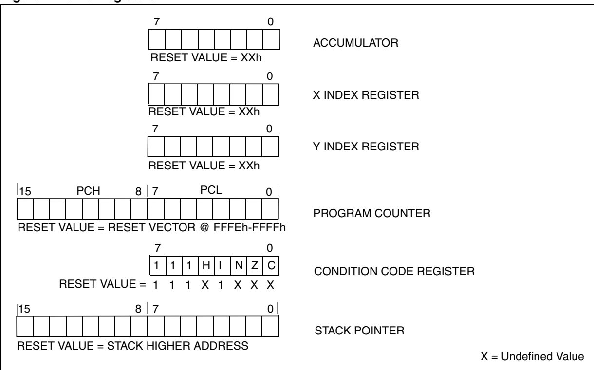
Figure 11. CPU Registers
