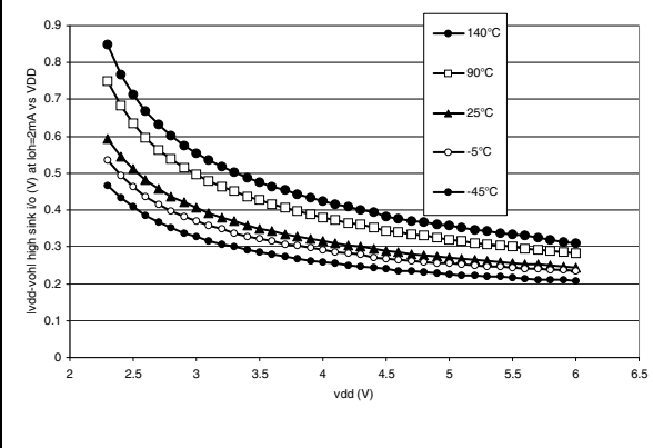
Figure 104. Typical V_{DD}-V_{OH} vs. V_{DD} (PORT C)
