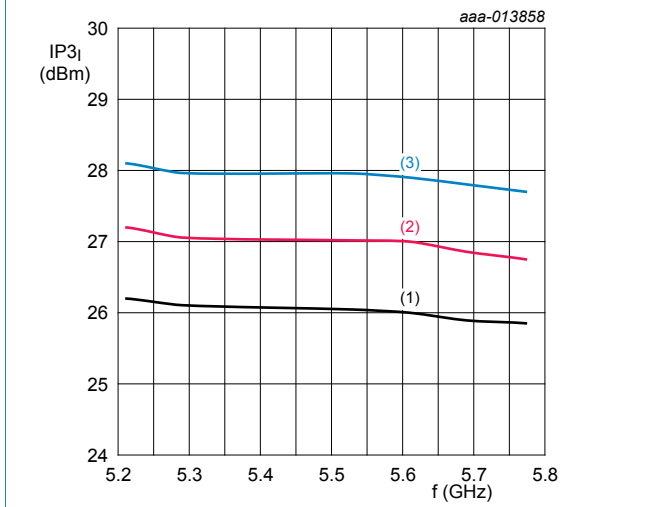
Figure 30. Input third-order intercept point as a function of frequency at different supply voltages
