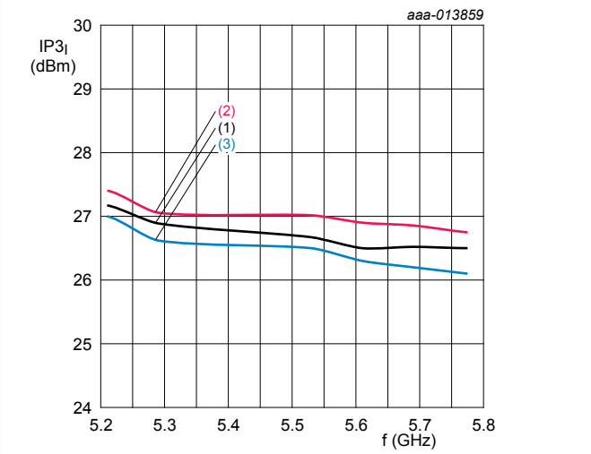
Figure 31. Input third-order intercept point as a function of frequency at different ambient temperatures
