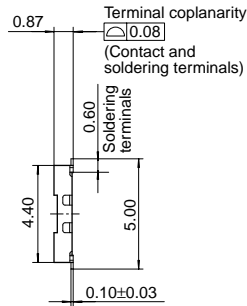
F-F cross section
