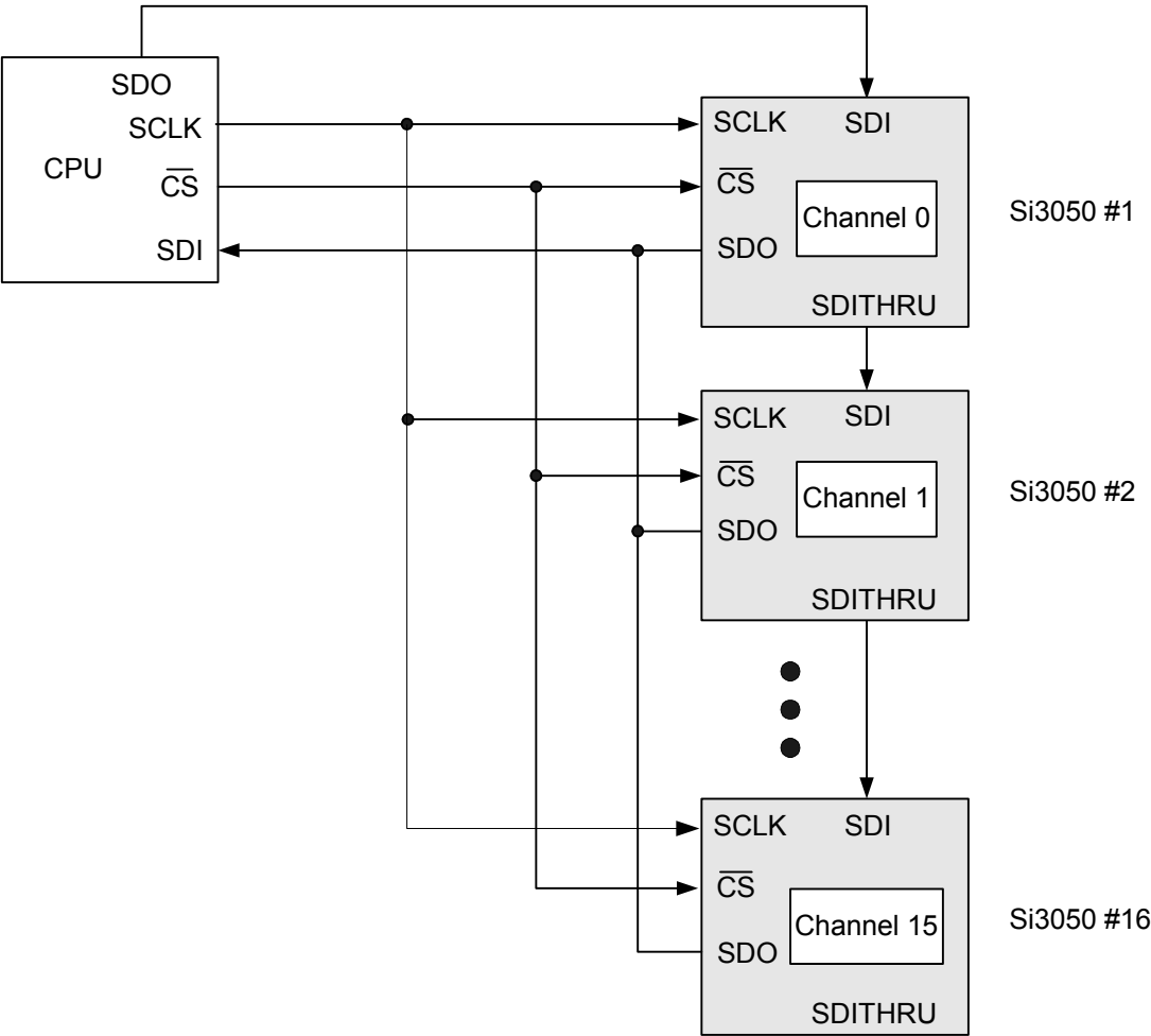
Figure 34. SPI Daisy Chain Control Architecture
