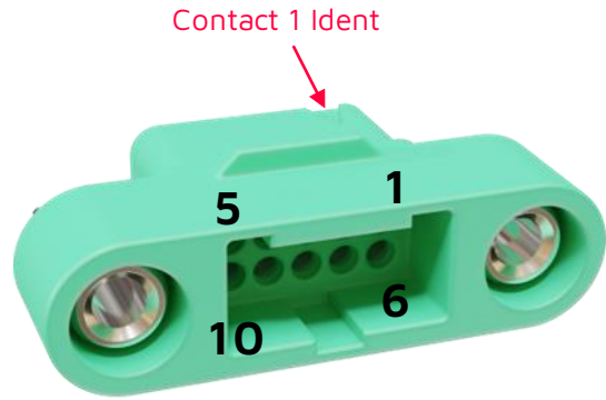
Male Crimp Housing
