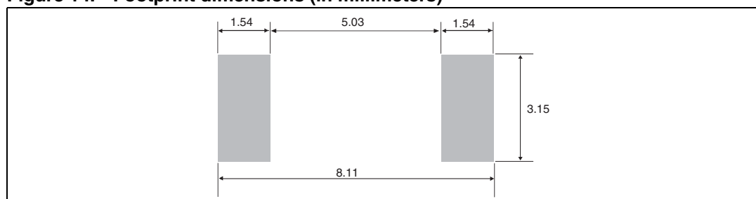
Figure 14. Footprint dimensions (in millimeters)
