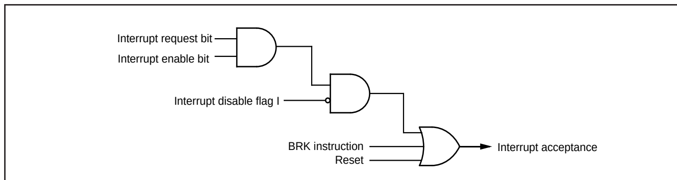
Fig. 17 Interrupt control
