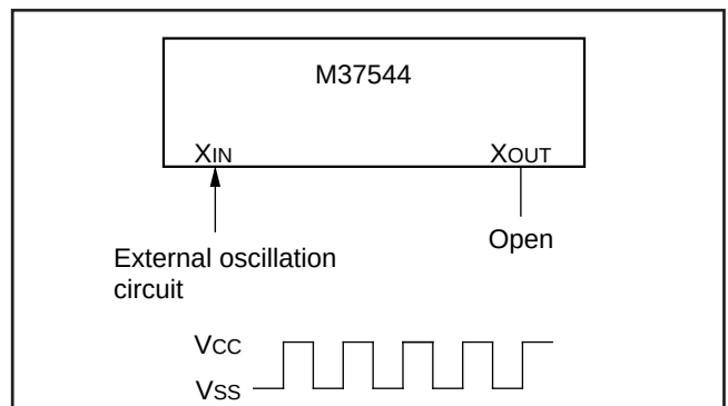
Fig. 44 External clock input circuit
