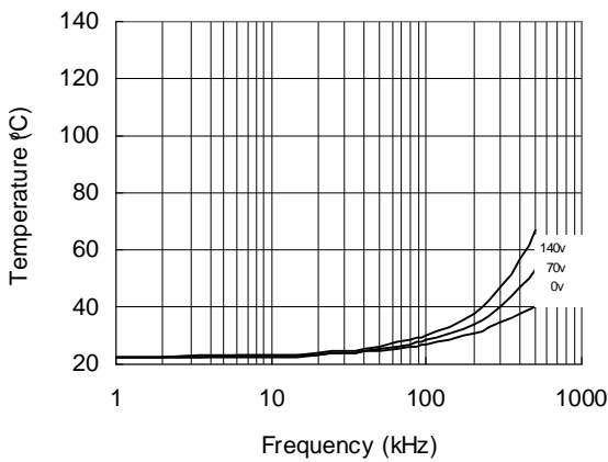
Figure 39. IRS21844 vs. Frequency (IRFBC30), R_{gate} = 22\Omega , V_{cc} = 15V
