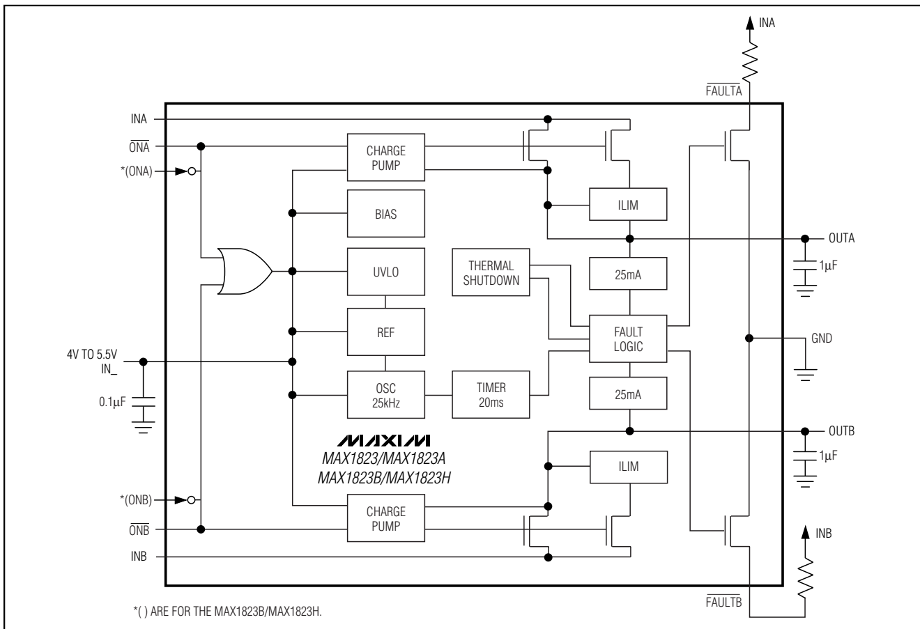
Figure 2. Functional Diagram
