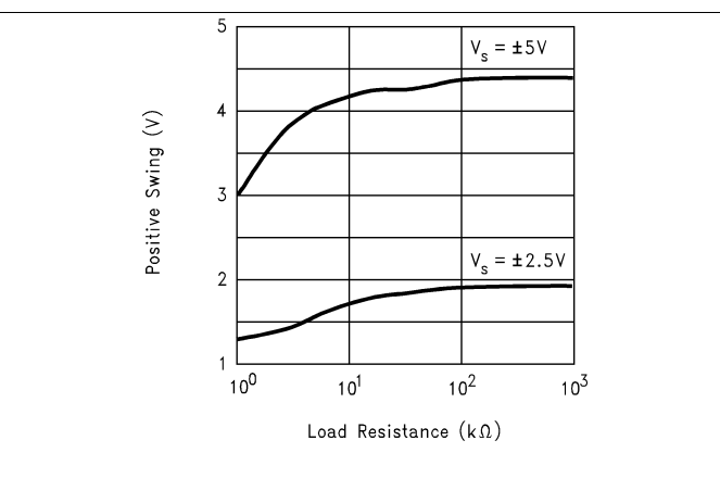
Figure 6. Positive Output Voltage Swing vs Load Resistance
