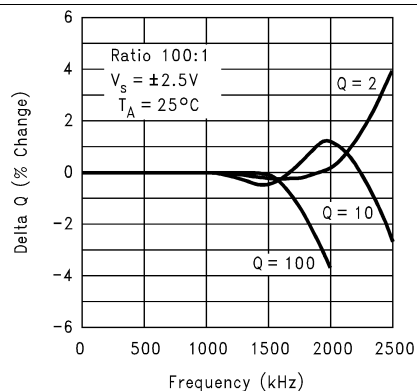
Figure 16. Q Deviation vs Clock Frequency
