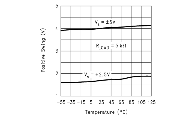
Figure 4. Positive Output Swing vs Temperature
