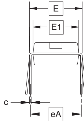
End View
