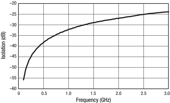
Figure 4. Average Isolation vs Frequency
