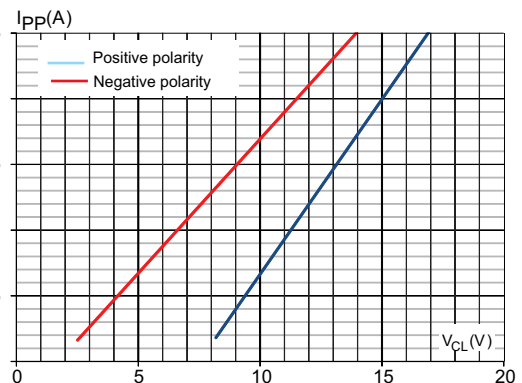
Figure 8. TLP measurements
